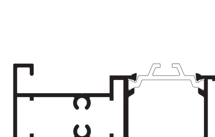
SPW63619 OVERSWING TRANSOM/MULLION
