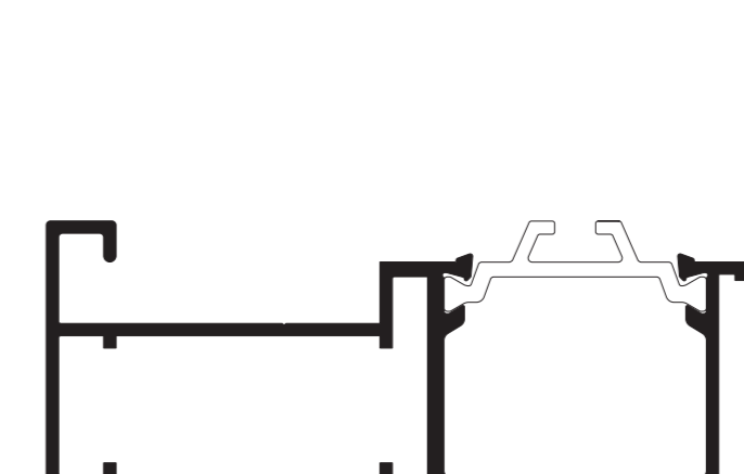
SPW63419 OVERSWING TRANSOM/MULLION
