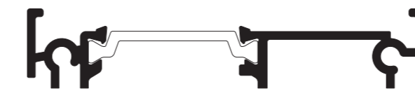
SPW66170 LOW THRESHOLD OPEN IN
