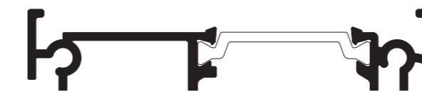
SPW67061 LOW THRESHOLD OPEN OUT
