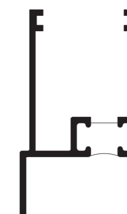
SXTW204 28mm VENTILATOR CARRIER
