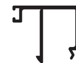
SPW624 32mm INT. GLAZED BEAD
