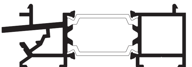
SPW68553 DRAINAGE CILL
