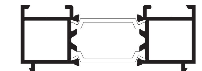
SPW65353 25mm ADD-ON
