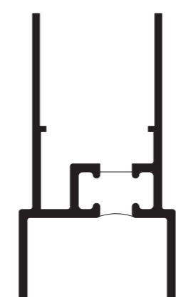
SX203 24mm VENTILATOR CARRIER
