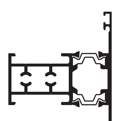
SPW31913 Transom/Mullion
