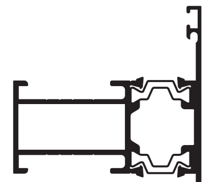
SPW31013 Transom/Mullion
