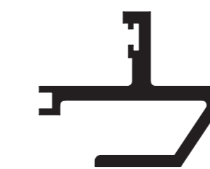
SFG136 REBATE DOUBLE GLAZED
