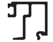
SD548 OFFSET SG BEAD
