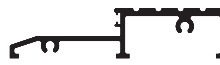
SD502 REBATED THRESHOLD
