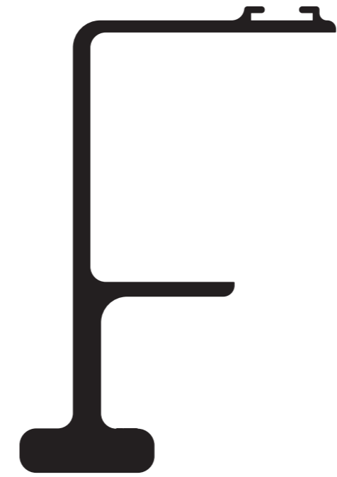
SD605 VERTICAL HANDLE / REINFORCING
