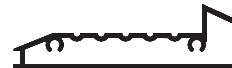
SD503 DRAINED THRESHOLD
