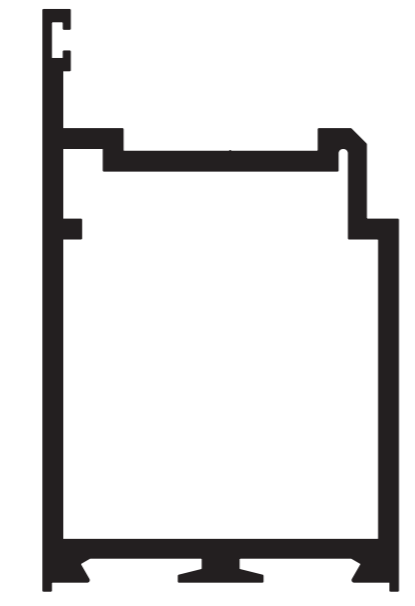
SD565 REBATED DOOR STILE
