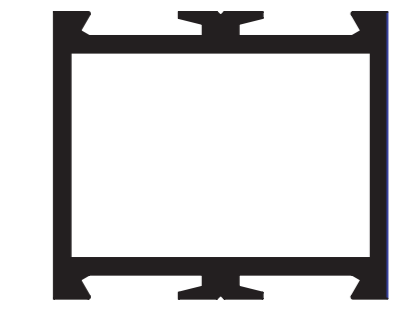
SD569 MIDRAIL
