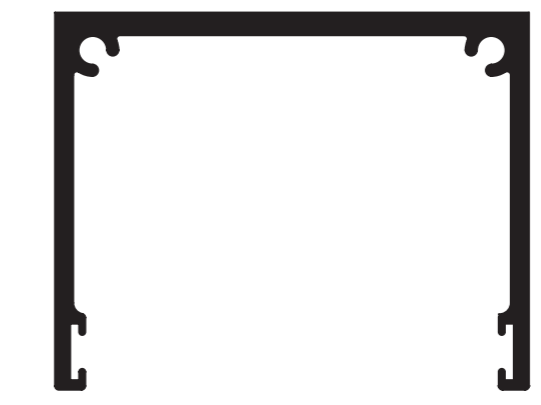
SD607 50mm DEEP GUIDE CHANNEL
