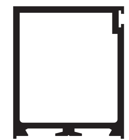
SD555 DOOR WEATHERSTRIP STILE
